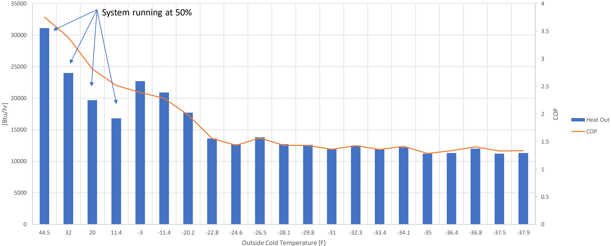
Heat Pump: Heat Out and COP vs Cold Outside Temperature
